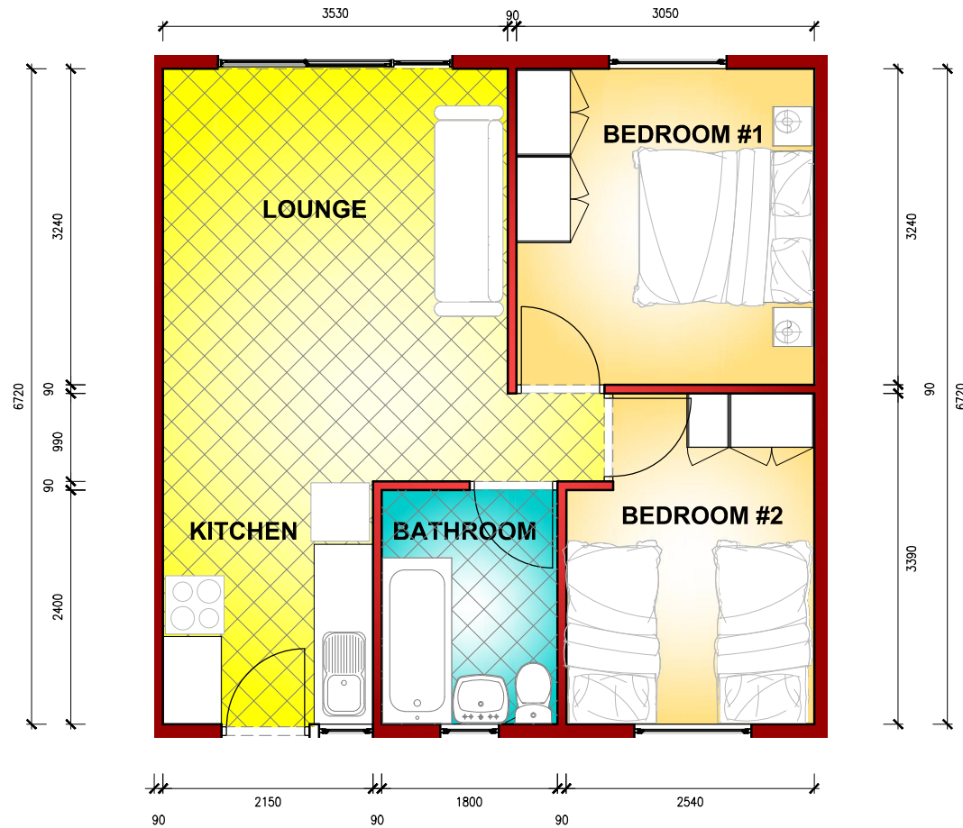
BLOCK C TYPICAL 2 BEDROOM UNIT
